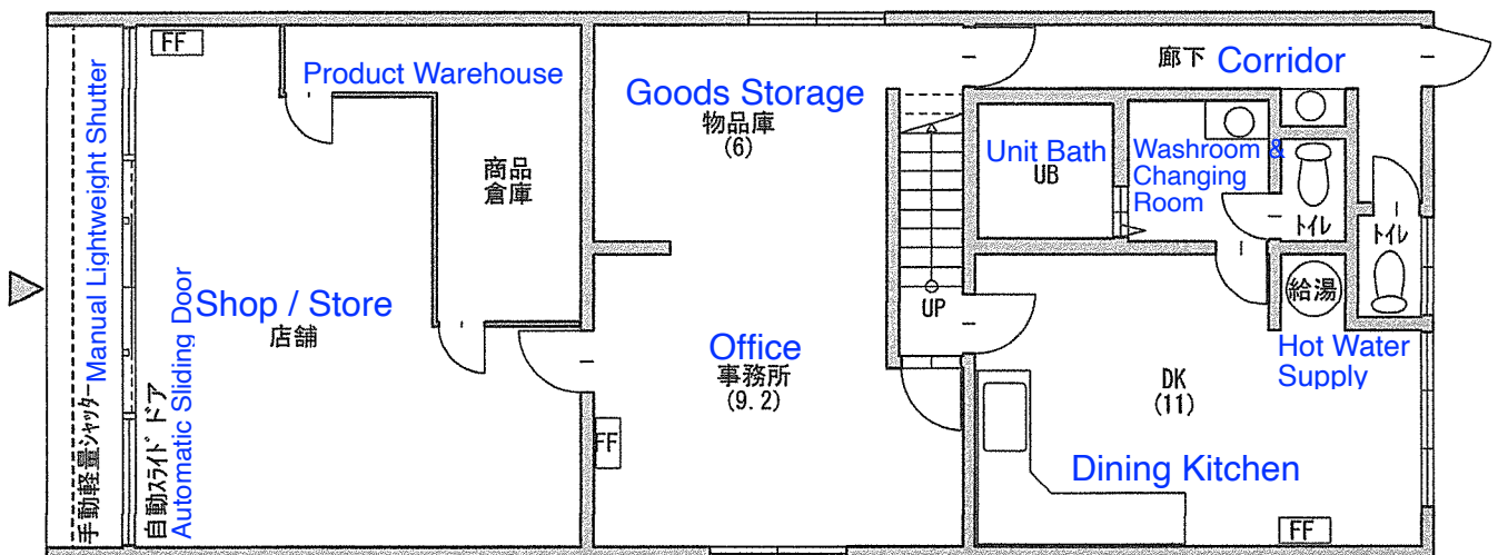
1st Floor Plan 1階平面図 S=1/100 (29.7坪)
