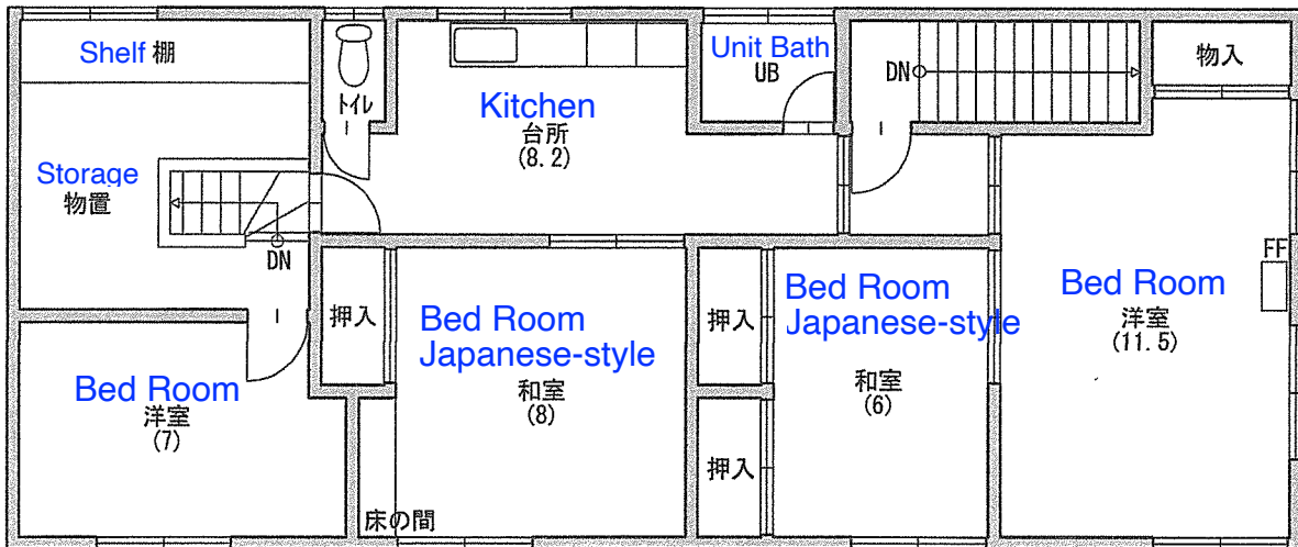
2nd Floor Plan 2階平面図 S=1/100 (29.7坪)
